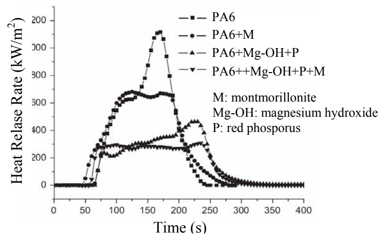
Fig.1. Distribution of heat generation with different additives in PA6 [17]
